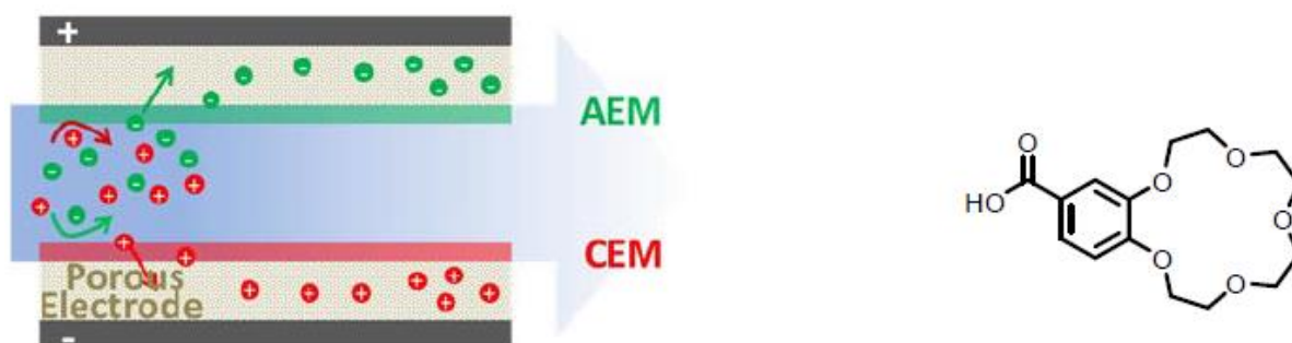
Figure 1. (left) Schematic representation of capacitive deionization with anion and cation-exchange membranes (AEM and CEM, respectively) and (right) the structure of an \text{Na}^+ -selective molecule that will be used to functionalize the porous electrodes.
